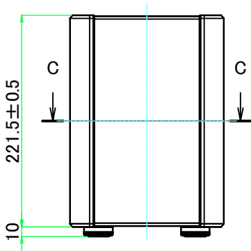
A view
